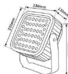
NO:YF-FX-05 48W 5865 Outer diameter size: 230x230MM Inner diameter: 193x193MM Power: 48W Shell material: die cast aluminum
