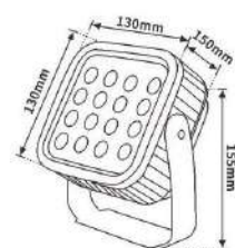
NO:YF-FX-02 16W 2415 Outer diameter size: 130x130MM Inner diameter: 95x95MM Power: 16W Shell material: die cast aluminum
