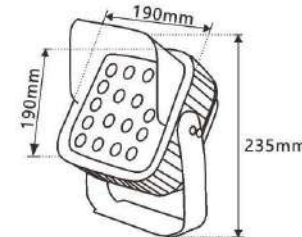
NO:YF-FX-09 24W 3795 36W 4255 Outer diameter size: 190x190x235MM Inner diameter: 155x155MM Power: 24W/36W Shell material: die cast aluminum
