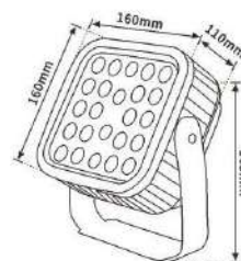
NO:YF-FX-03 18W 2875 24W 3175 Outer diameter size: 160x160MM Inner diameter: 125x125MM Power: 18W/24W Shell material: die cast aluminum
