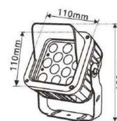
NO:YF-FX-06 9W 1955 12W 2120 Outer diameter size: 110x110x150MM Inner diameter: 85x85MM Power: 9W/12W Shell material: die cast aluminum
